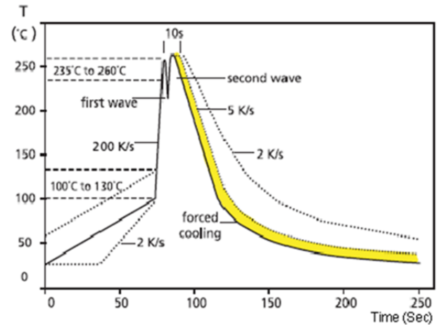
Recommended double-wave Soldering Profile
